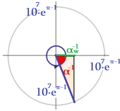
Figure 5. The angle in a^{-1} radians. The rotation vector moves in a circle of radius 10^7 \cdot e^{n-1} .
