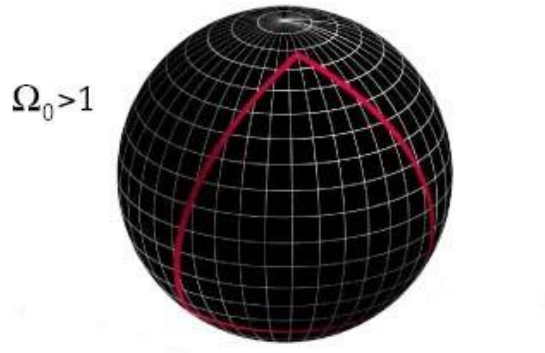
Figure 16. If \Omega_0 is greater than 1, the Universe is closed and this will eventually halt its expansion and recollapse.
