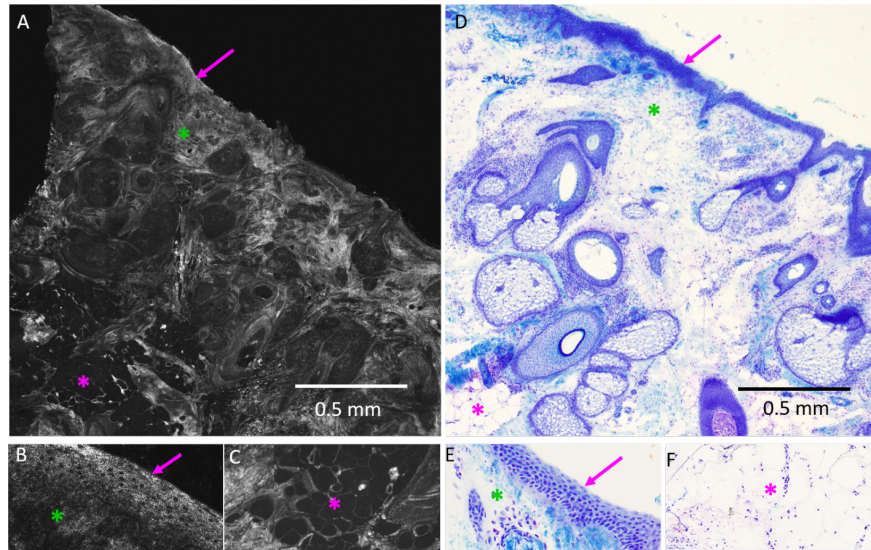
Figure 1. Images of normal layers of the skin. (A) FF-OCT image showing grayish epidermal lining (pink arrow), dermis (green asterisk), and underlying subcutis (pink asterisk). (B) A stratified layer of the epidermis (pink arrow) shows multiple round to oval dark nuclei surrounded by bright (grayish) cytoplasm. The underlying dermis appears grayish (green asterisk). (C) Adipocytes of the subcutis appear as dark polygonal structures separated by thin white septa (pink asterisk). (D-F) Corresponding histopathology section stained with Toluidine blue. Magnifications: (A) = 5.2 mm x 5.2 mm; (B, C) = 300 x 150 mm; (D)= 10x; (E, F) = 40x .
